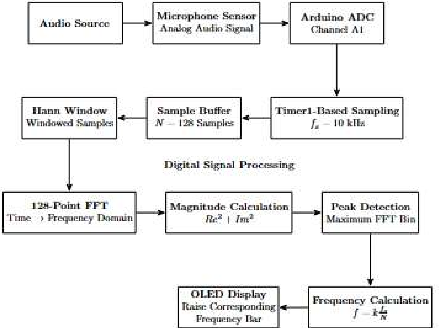
Figure 1: Block diagram of the Arduino-based real-time audio spectrum analyzer
